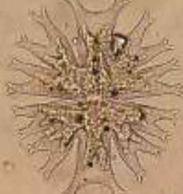
Micrasterias radians
