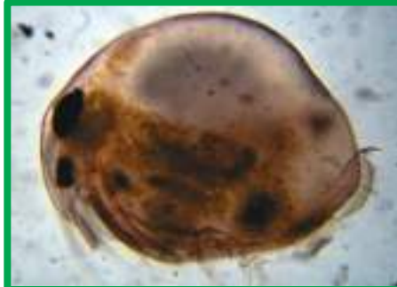
Dadayia macrops
